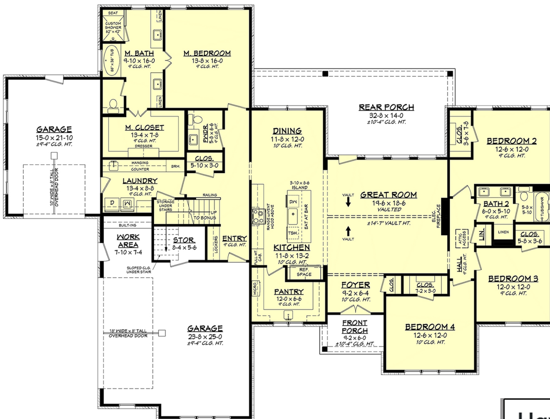
Floor Plan
