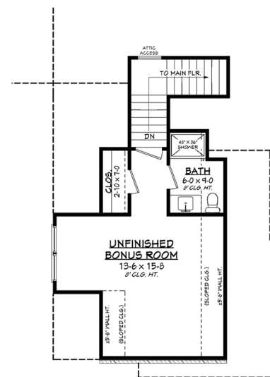
Bonus Floor Plan
