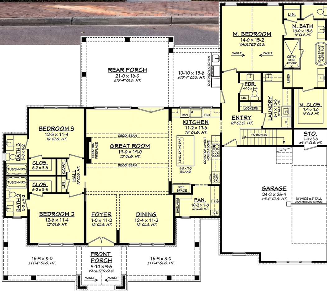
Floor Plan
