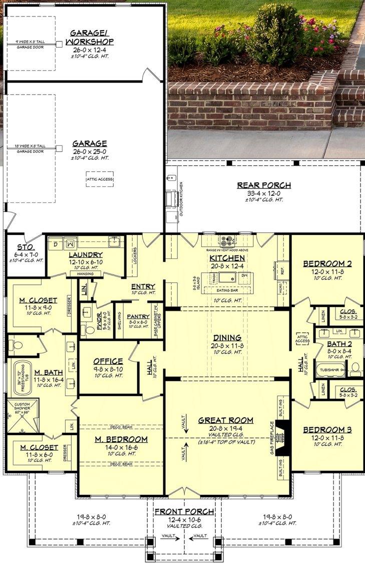
Floor Plan
