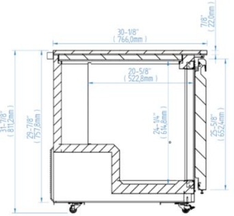
RIGHT VIEW
