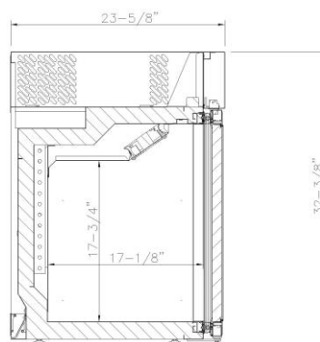
RIGHT VIEW
