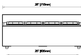
CPR-60-4 Front View
