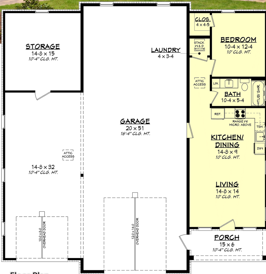
Floor Plan
