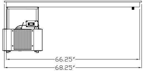
Exhaust side
