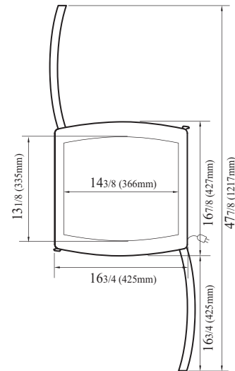
PLAN VIEW
