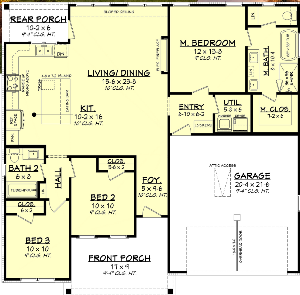
Floor Plan
