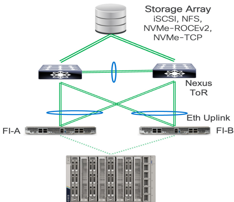
Figure 23 IP-SAN Connectivity with Cisco UCS Fabric Interconnect 9108 100G and Appliance Port through ToRs in vPC Port Channel configuration
