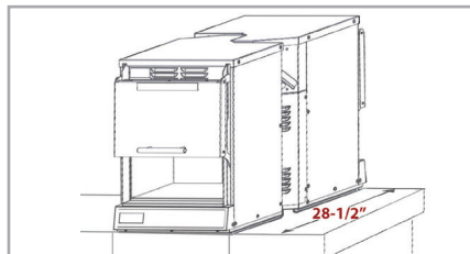
Two units fit back-to-back on a 28 ½" (724 mm) shelf in a 13 ⅝" (346 mm) space
